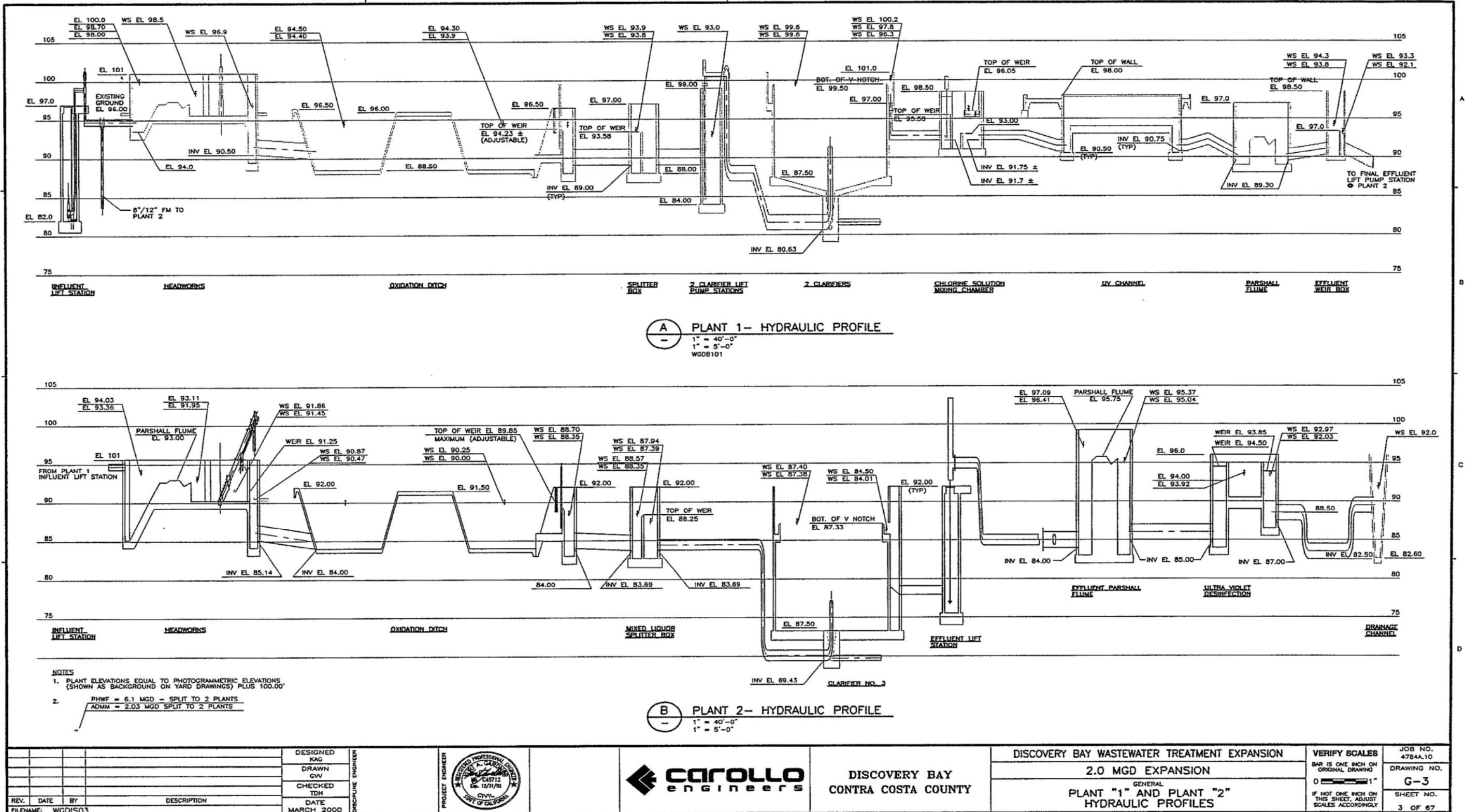
Figure 6-2 Hydraulic Profile
